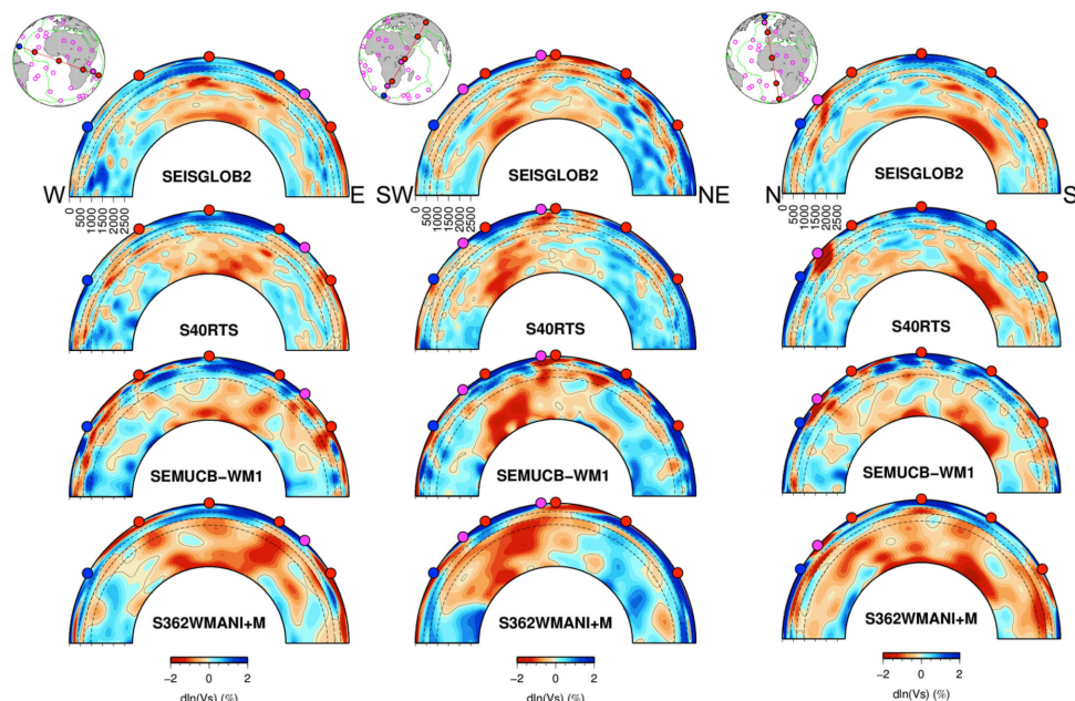
Figure 8. Same as Fig. 7, but below Atlantic and Africa.
