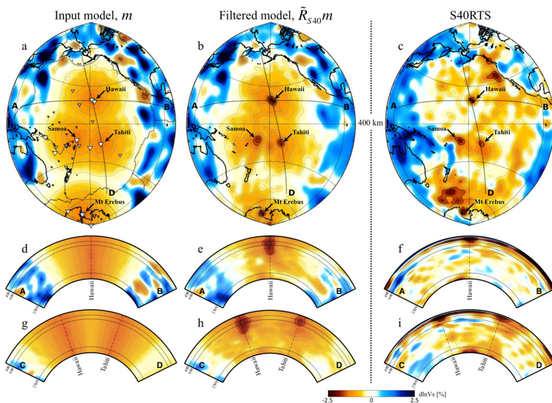
Figure 3. Quantitative illustration of the local averaging bias effect in model S40RTS. (a, d, g) Input model, \mathbf{m} ; (b, e, h) filtered model, \tilde{\mathbf{R}}_{S40}\mathbf{m} ; (c, f, i) model S40RTS. In Figure 3a large-size white (medium-size gray, small-size black) triangles denote all receivers located within the Pacific or Antarctica regions for which there is a large (moderate, small) number of recorded body wave arrival times in S40RTS data set, respectively.
