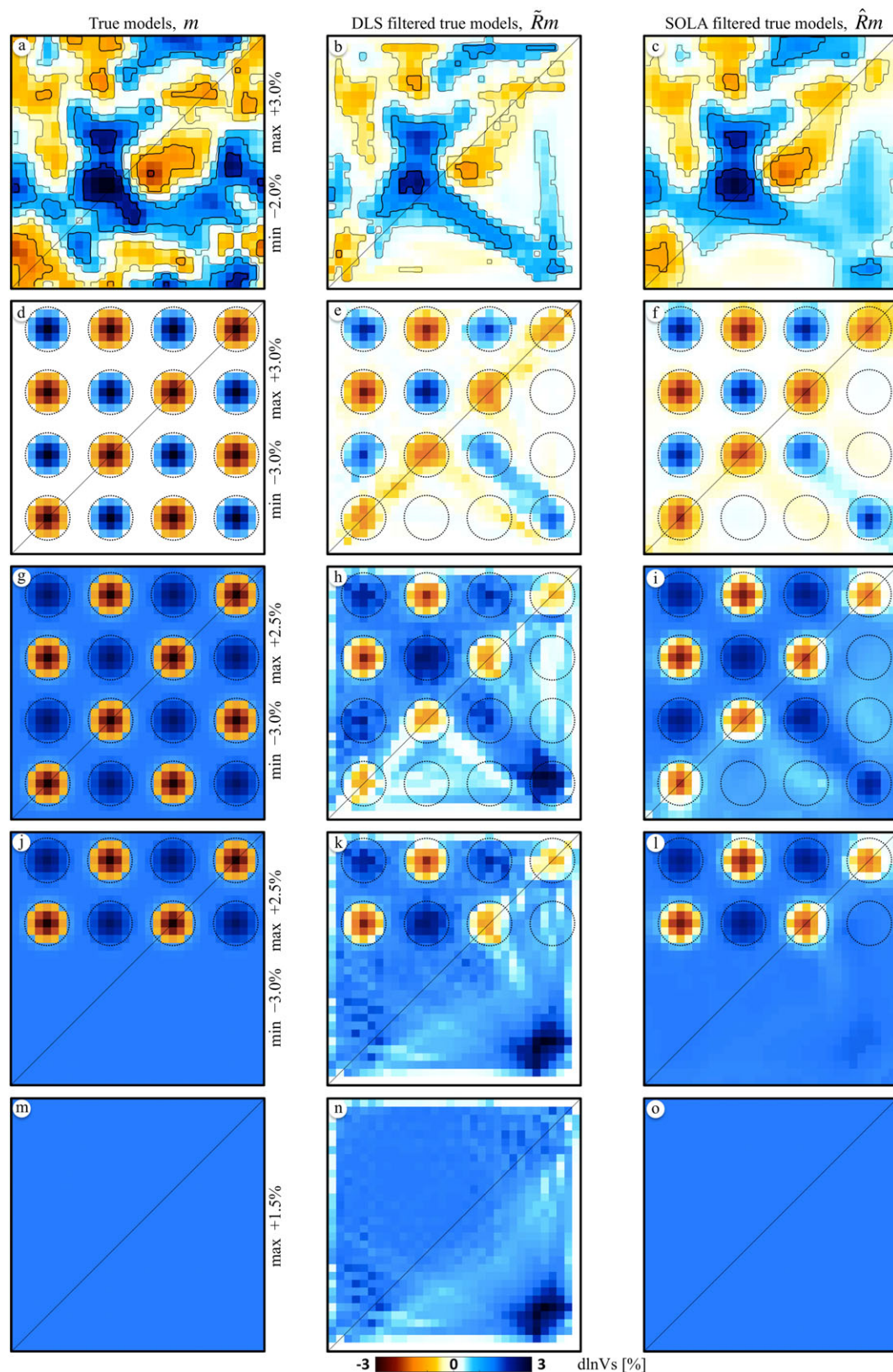
Figure 2. Toy problem. (a, d, g, j, m) True models, m (minimum and maximum values are indicated); (b, e, h, k, n) DLS filtered true models, \tilde{R}m ; and (c, f, i, l, o) SOLA filtered true models, \hat{R}m . Anomalies of the first true model (Figure 2a) are spatially distributed like a 2-D Gaussian random field.
